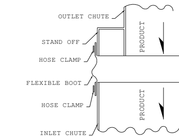
Round or elliptical boot connection with hose clamp
